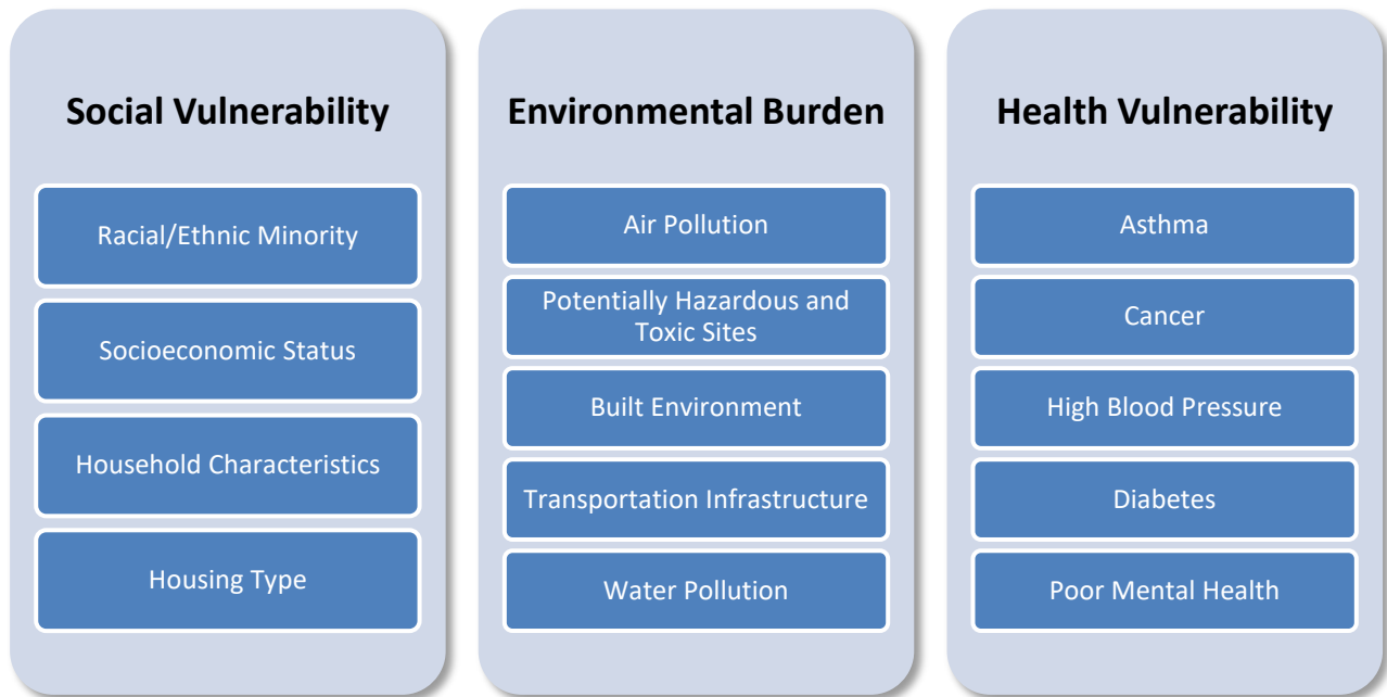
Figure 19: EJI Variables
